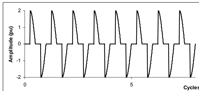
c) Harmonic test current, zero current during phase angles of 0-90° and 180-270°.
