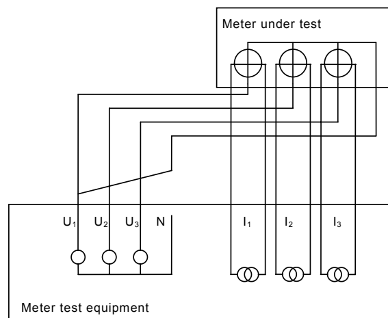
Figure 5. Set-up for earth fault test.
