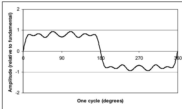
Figure 1. Current amplitude for quadriform waveform.
