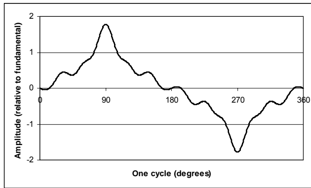
Figure 2. Current amplitude for peaked waveform.
